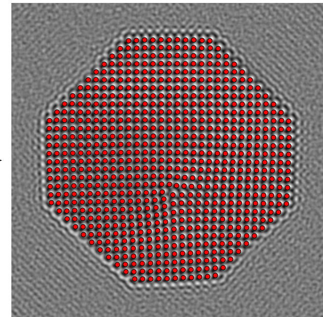
Identified positions of atomic columns
