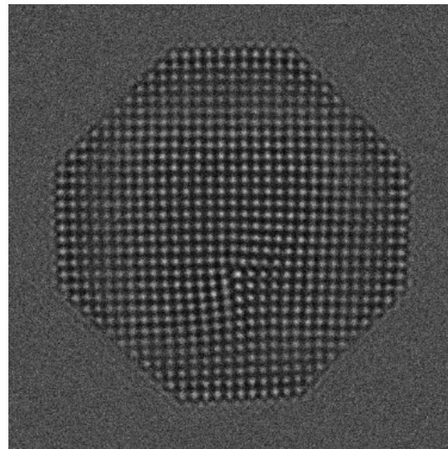
Noisy simulated HRTEM image
